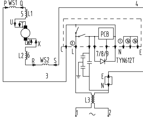
Electric Circuit
